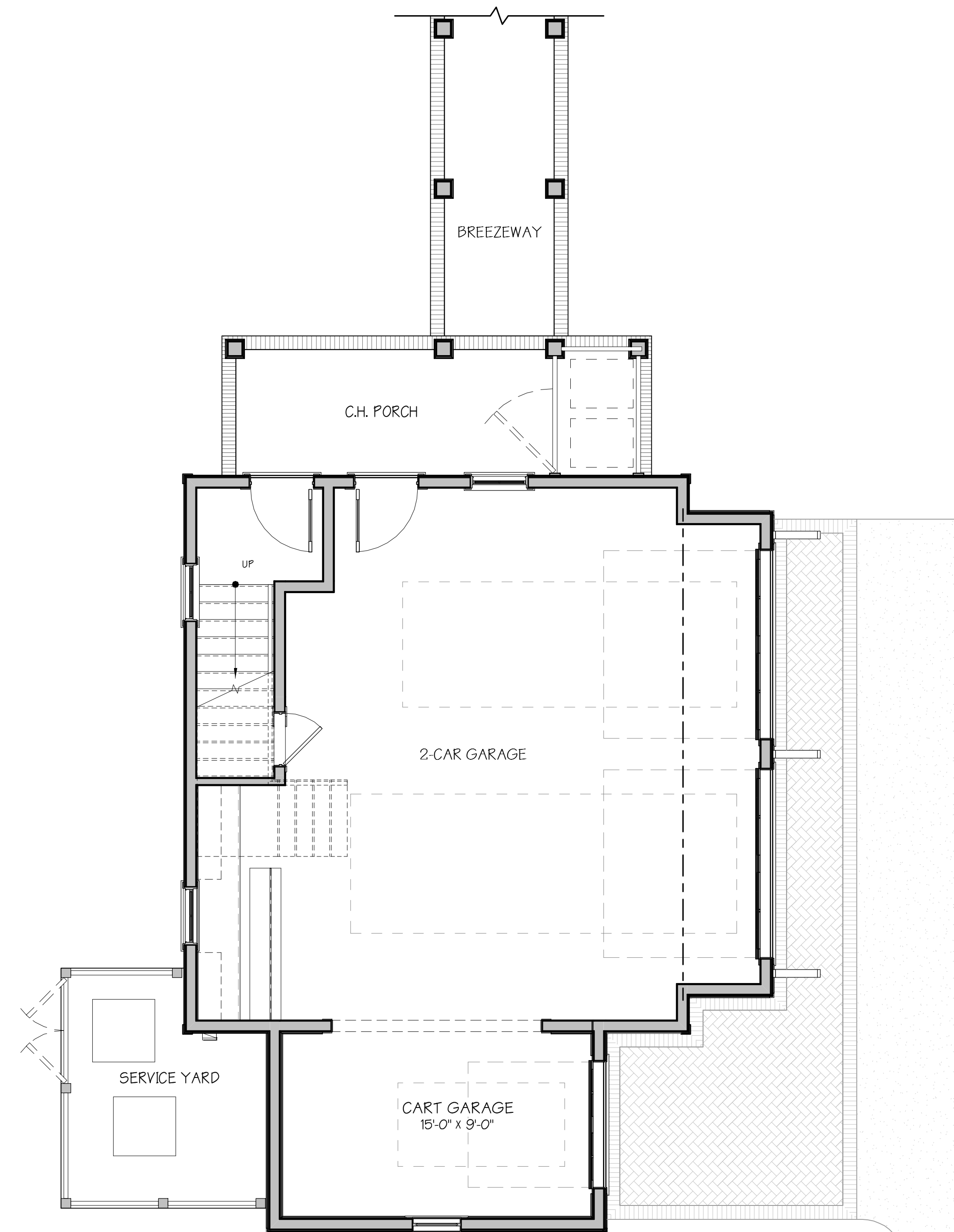
C.H. FIRST FLOOR PLAN
