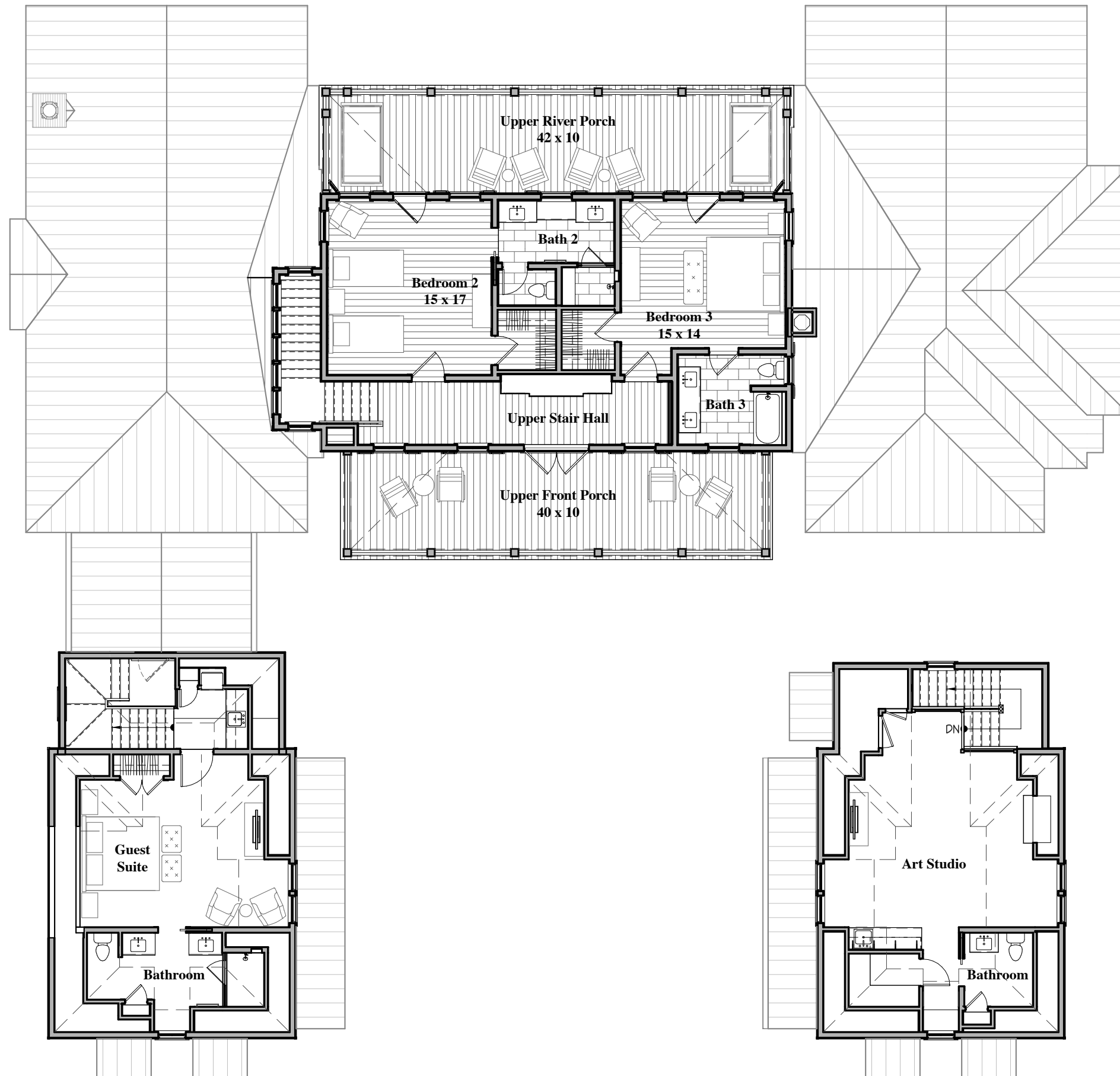
Second Floor Plan // 3/32" = 1'-0"
