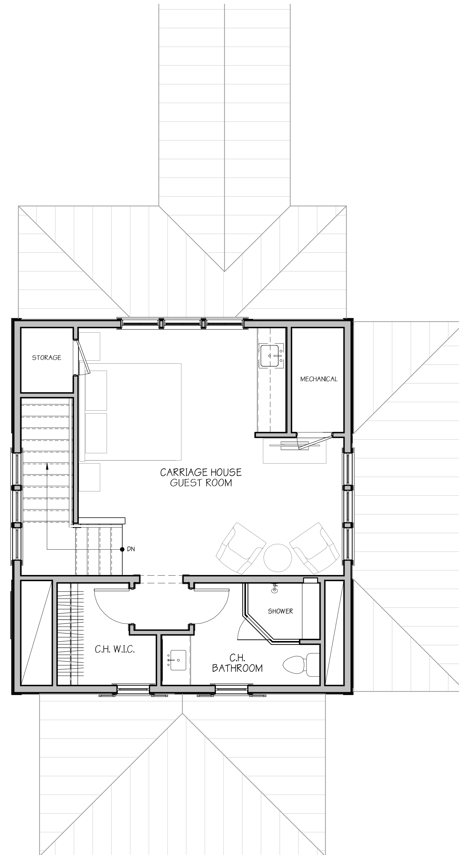
C.H. SECOND FLOOR PLAN
