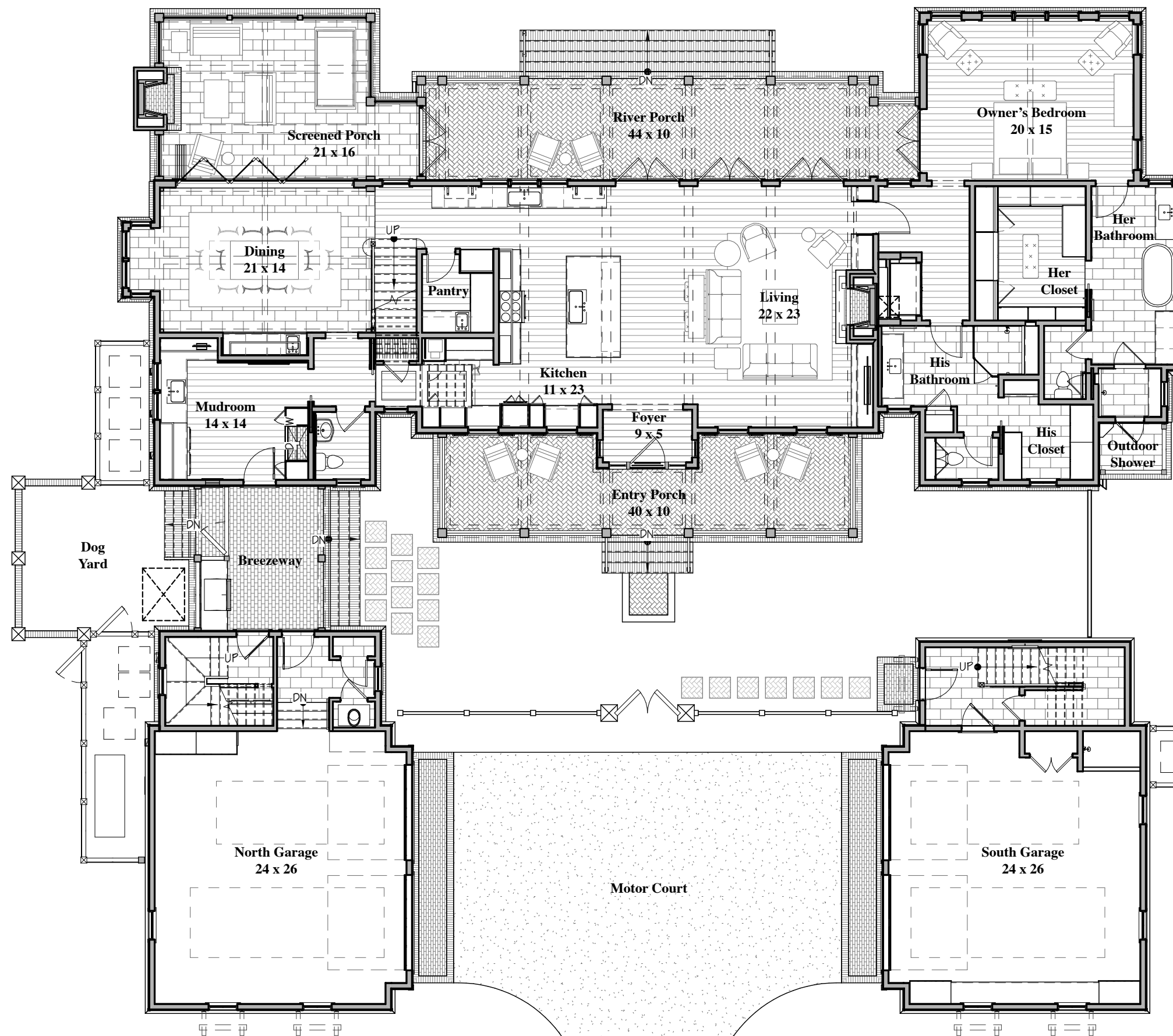
First Floor Plan // 3/32" = 1'-0"
