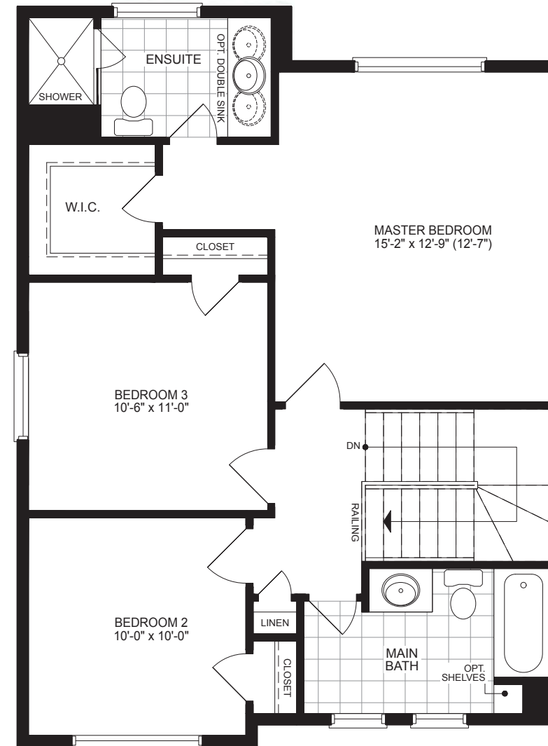
SECOND FLOOR PLAN ELEVATION A & B
