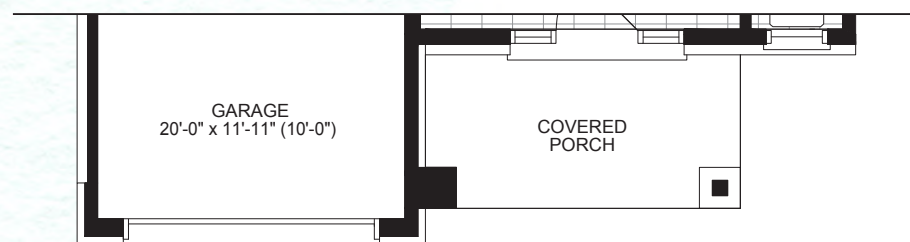
PARTIAL GROUND FLOOR PLAN ELEVATION B
