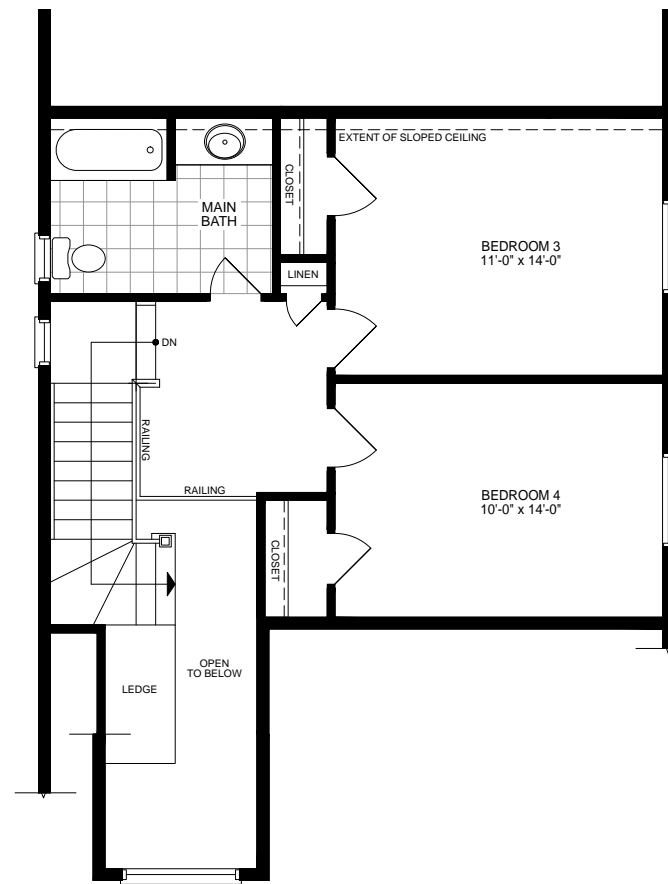
ALT. SECOND FLOOR PLAN ELEVATION A & B
