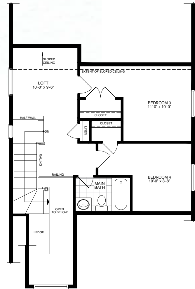
SECOND FLOOR PLAN ELEVATION A & B
