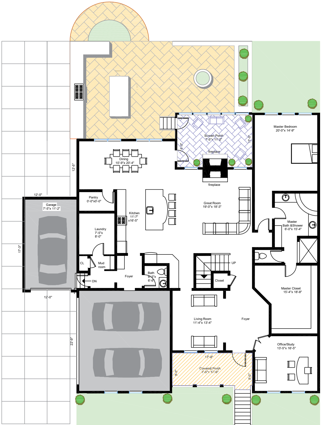
1st. Floor
