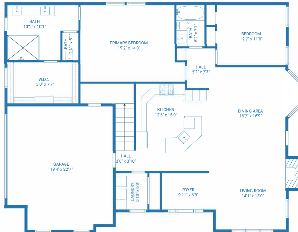
FLOOR 1
