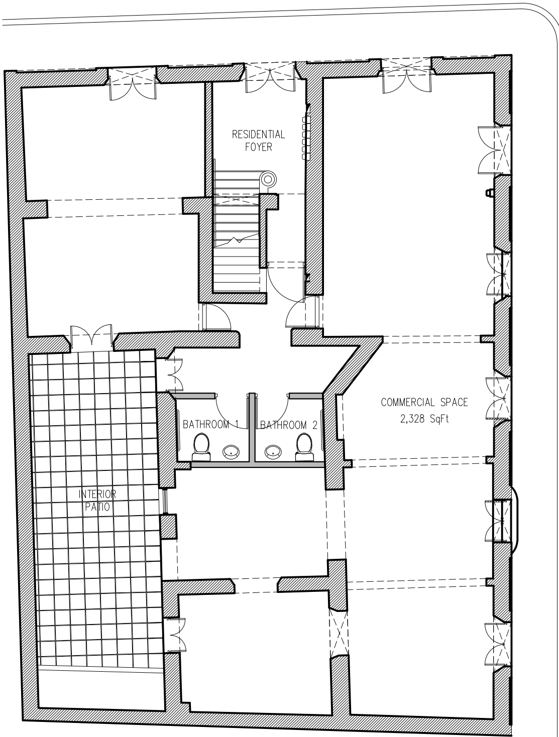
ground floor plan | commercial space
